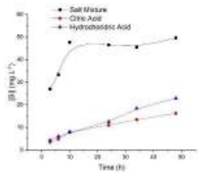
Figure 2. Release curves for Si using extracts solutions
